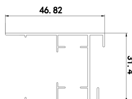
Outer Frame
