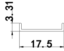
Cover Plate
