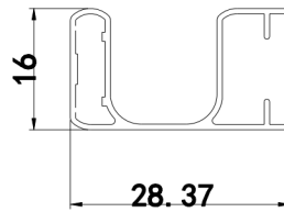
Sliding Bar
