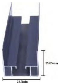
Outer Fame
