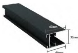
Outer Fame
