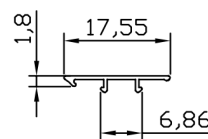
Cover Plate
