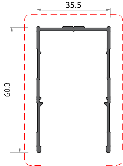
Screen Housing Cover AL-S39376
