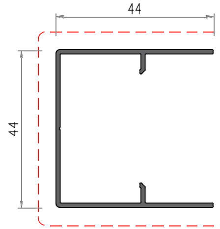
Housing AL-S45740
