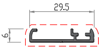
Catch Frame AL-S39377
