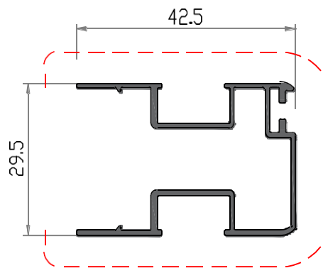
Sliding Bar AL-S39375
