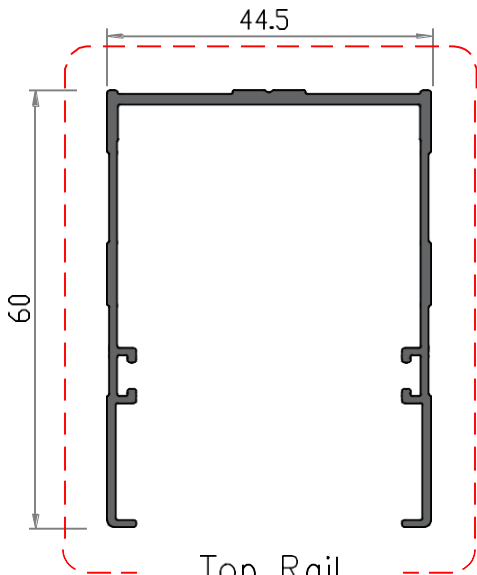
Top Rail AL-S39378
