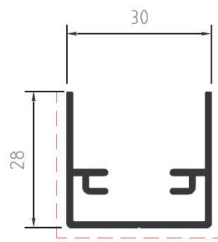
Housing 28
