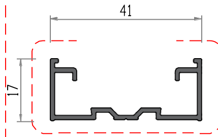
Bottom Rail AL-S45744
